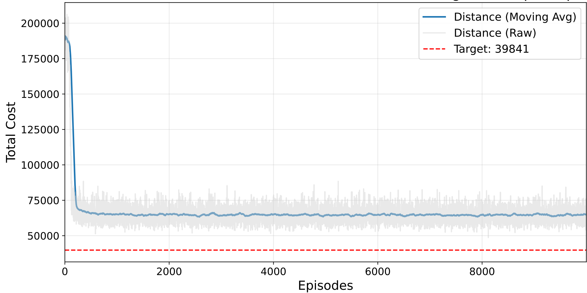
Final GAUSSIAN PROCESS Masked AutoRL-SOP Training - kro124p.2.sop
